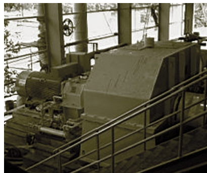
View of the cane mill (862 kW)
